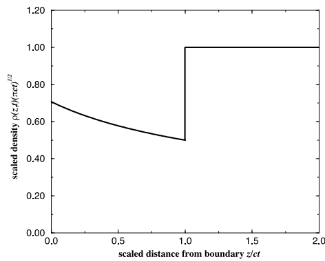
Figure 7. The late-time scaled density profile near the boundary.
