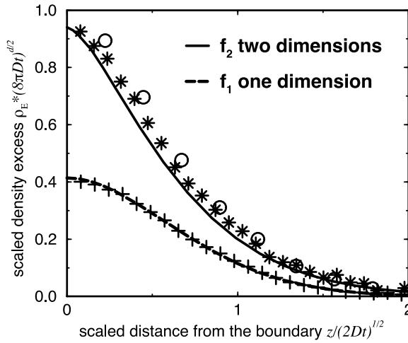
Figure 3. The density excess in one and two dimensions, f_1 and f_2 . The RG results are compared with simulations at time t = 10 ( \circ ) and t = 80 ( * ). The exact results f_1 calculated for infinite reaction rate is compared with simulations for finite reaction rate \lambda = \frac{1}{2} ( + ) demonstrating the universality.
