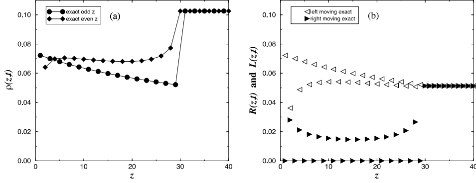
Figure 6. An example of the exact (a) density profile and (b) densities of left and right moving particles at time t = 30 . The difference between odd and even sites becomes increasingly less pronounced at later times.
