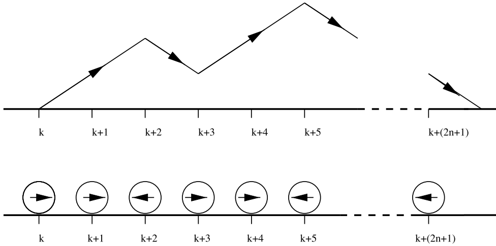
Figure 4. An illustration of the mapping to the ballot problem. The arrows, representing the direction a particle is moving, are considered as moves of a random walker as illustrated above.
