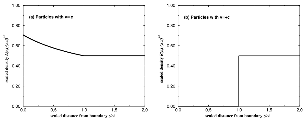
Figure 8. The late-time scaled density of (a) left-moving particles with v = -c and (b) right-moving particles with v = +c .
