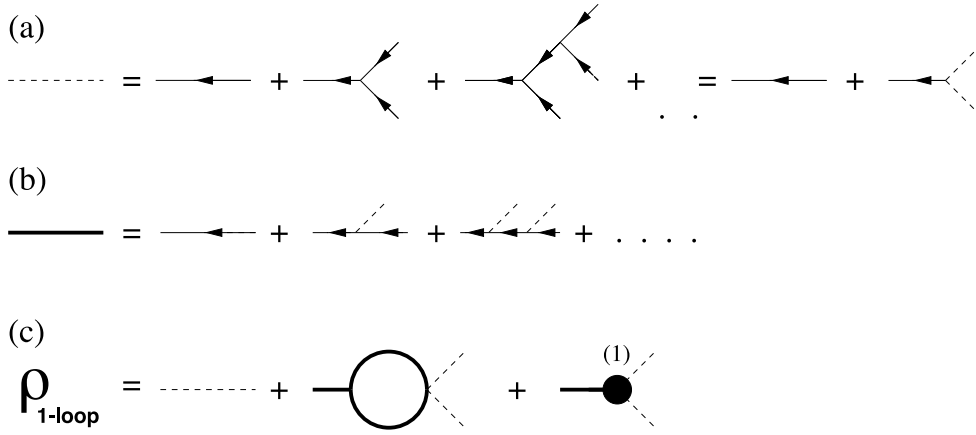
Figure 2. The diagrammatic representations of (a) the tree-level density calculation, (b) the classical propagator and (c) the perturbative density to the level of one loop, which reading from left to right are \varrho^{(0)} , \varrho^{(1)} and \varrho_{ct}^{(1)} .
