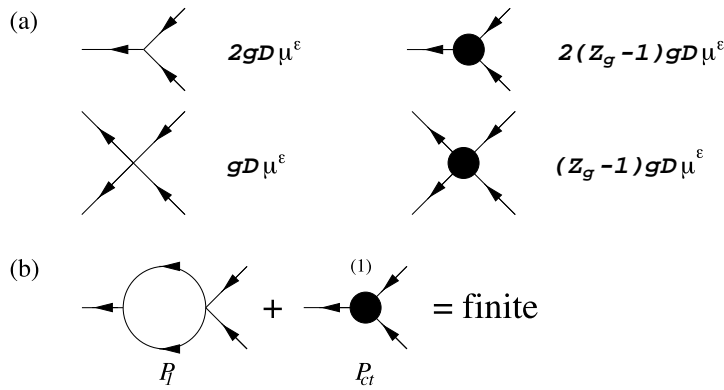
Figure 1. The diagrammatic representations of (a) the interactions and counter terms (with blob) and (b) the one-loop regularization. The propagator is denoted by a straight line with an arrow signalling the time direction. In the diagrammatic equation (b) P_1 and P_{ct} are the one-loop and Z_g^{(1)} counter-term contributions, respectively.
