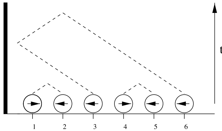
Figure 5. An example of the initial conditions studied. The numbers mark lattice sites, and dashed lines represent the trajectories of the particles.
